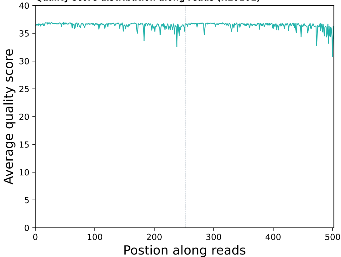
Quality score distribution along reads (R10101)
